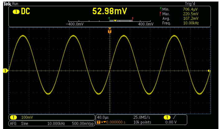
A DC measurement value is shown with a five second variation along with minimum, maximum, and average voltage values. The frequency of the waveform is also shown.
